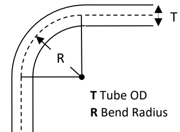
Figure 1 Recommended Bend Radius
